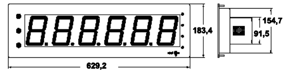
Dimensions (mm)
